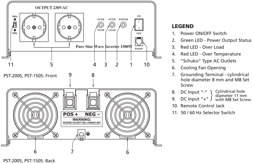
Fig. 6.3: Layout of PST-150S-12E, PST-150S-24E, PST-200S-12E, PST-200S-24E
