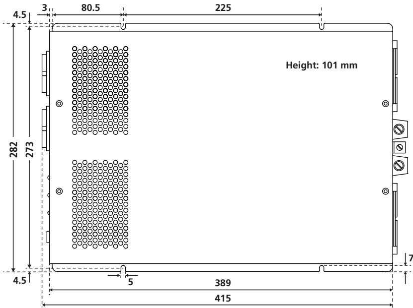
Fig. 8.3: Dimensions and Mounting Slots for PST-150S-12E, PST-150S-24E and PST-200S-12E, PST-200S-24E / Dimensions (mm): 282 x 415 x 101
