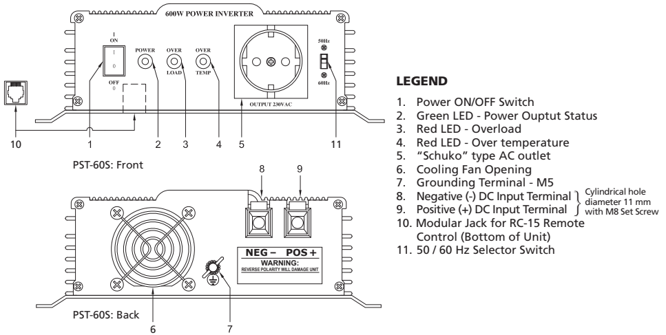
Fig. 6.1: Layout of PST-60S-12E, PST-60S-24E
