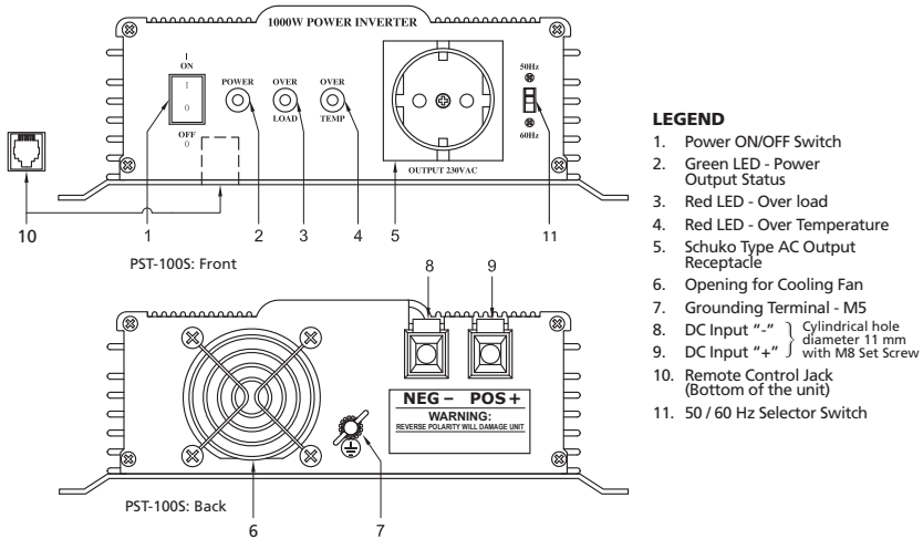
Fig. 6.2: Layout of PST-100S-12E, PST-100S-24E
