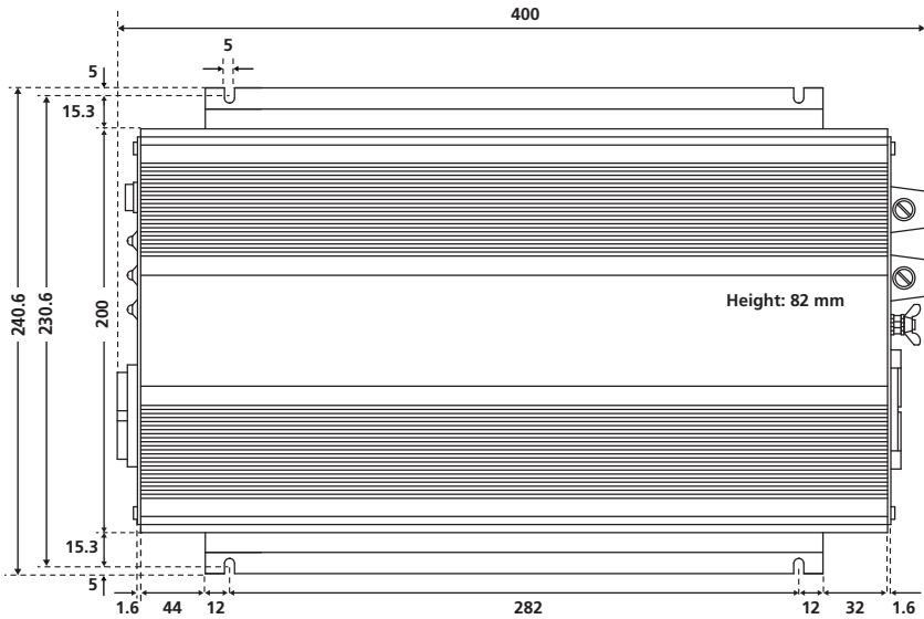
Fig. 8.2: PST-100S-12E, PST-100S-24E Dimensions and Mounting Slots / Dimensions (mm): 240.6 x 400 x 82
