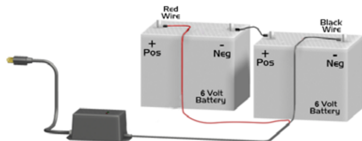
Two 12V Battery Connection
