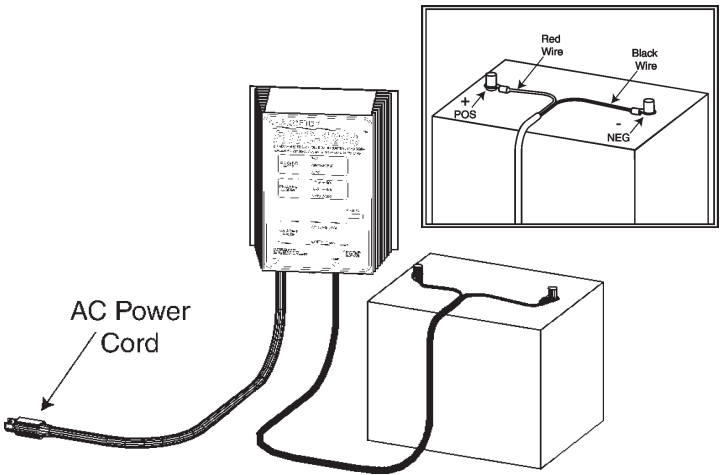
Single 12V battery connection
