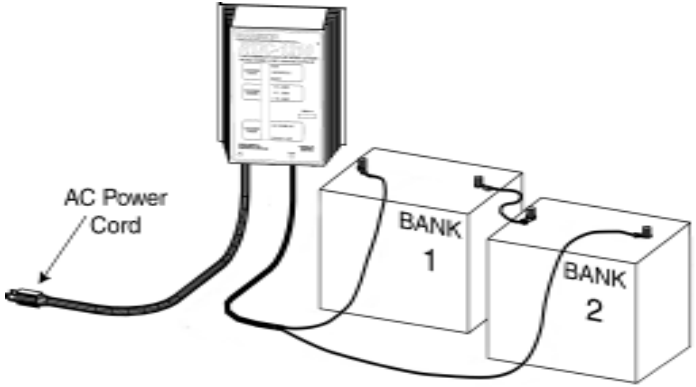
Two 6V battery connection
